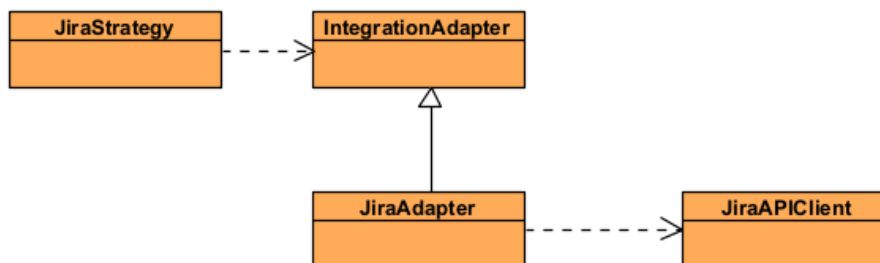
Figure 5: Adapter Pattern
