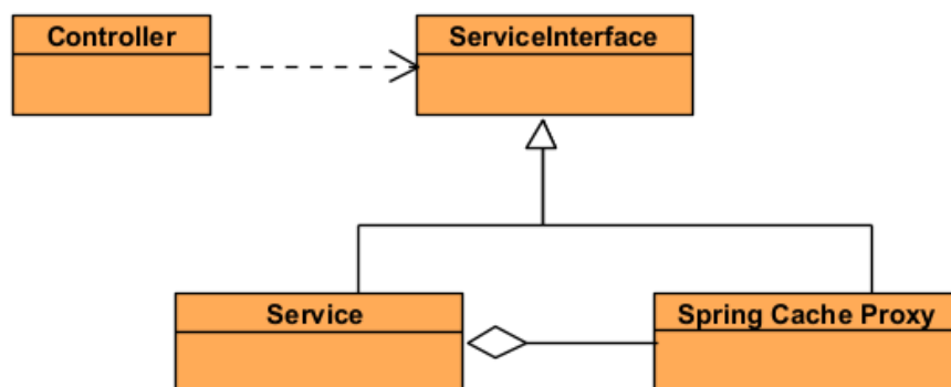
Figure 4: Proxy Pattern
